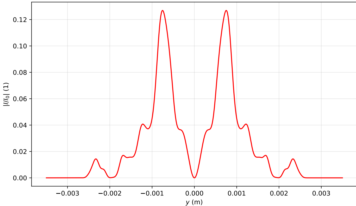
Intensity profile I(x=0, y, z=3.344)/I_0 , P_{in}=8.0P_{cr} , artificial time
